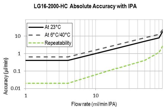
Figure 2: Flow meter accuracy and repeatability across the flow range. Relative error in % of measured value (left column) and absolute error in \mu\text{l}/\text{min} or \text{ml}/\text{min} (LG16-2000-HC) (right column) for IPA.
