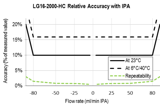
Figure 2: Flow meter accuracy and repeatability across the flow range. Relative error in % of measured value (left column) and absolute error in \mu\text{l}/\text{min} or \text{ml}/\text{min} (LG16-2000-HC) (right column) for IPA.
